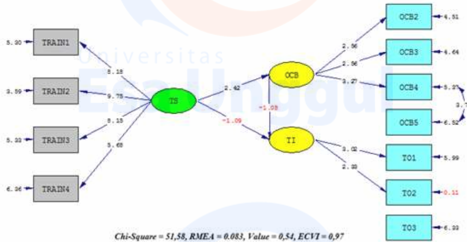
Gambar 2. Path Diagram T-Value
